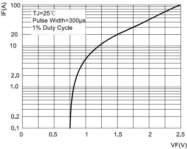
图6: 典型瞬时正向电压 FIG6: Typical Instantaneous Forward Voltage
