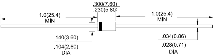
Dimensions in inches and (millimeters)
